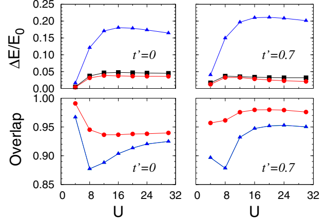
FIG. 1. (Color online) Results for 18 electrons on 18 sites as a function of U/t . Upper panels: Accuracy of energy \Delta E = (E_0 - E_v) , E_v , and E_0 being the variational and the exact values, respectively. Lower panels: Overlap between the exact ground state and the variational wave functions. The BCS state with long-range Jastrow factor is denoted by blue triangles, the BCS state with backflow correlations and Jastrow term by red circles. The results for \Delta E considering one Lanczos step upon the BCS state, i.e., (1 + \alpha\mathcal{H})|\Psi\rangle , are also shown (black squares).
